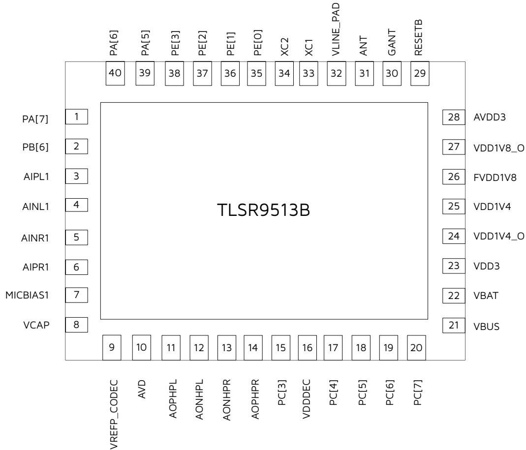
Figure 1-3 Pin Assignment of TLSR9513B
