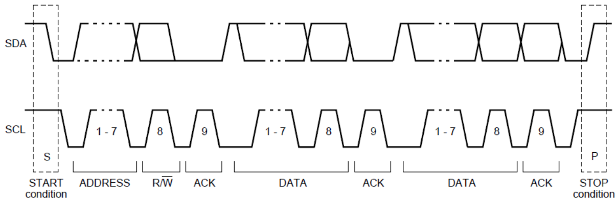
Figure 10-3 I2C Timing
