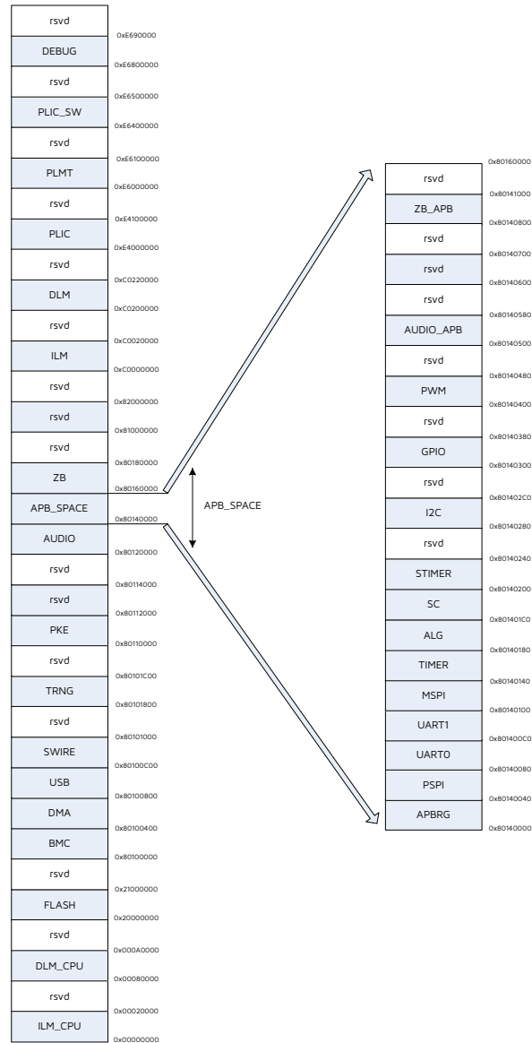
Figure 4-1 Memory Map
