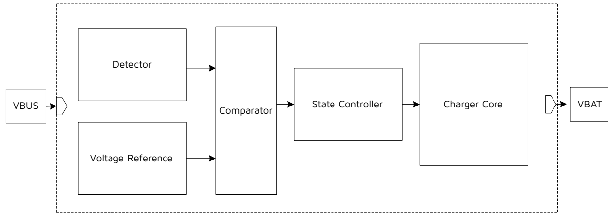
Figure 4-6 Charger Diagram
